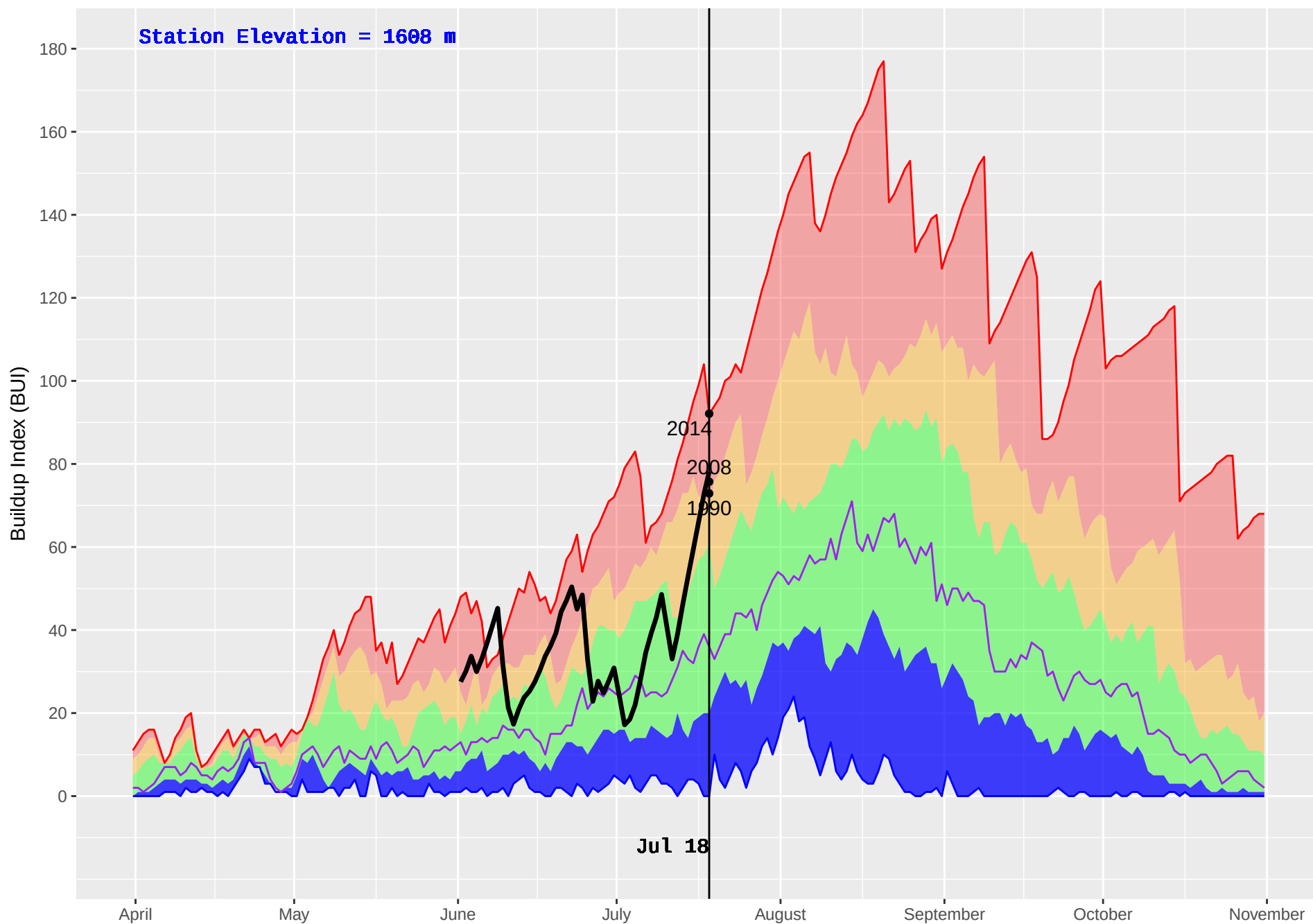
DEWAR CREEK (421) : Historical (1986–2016) and Current (2018) Daily Buildup Index (BUI)
