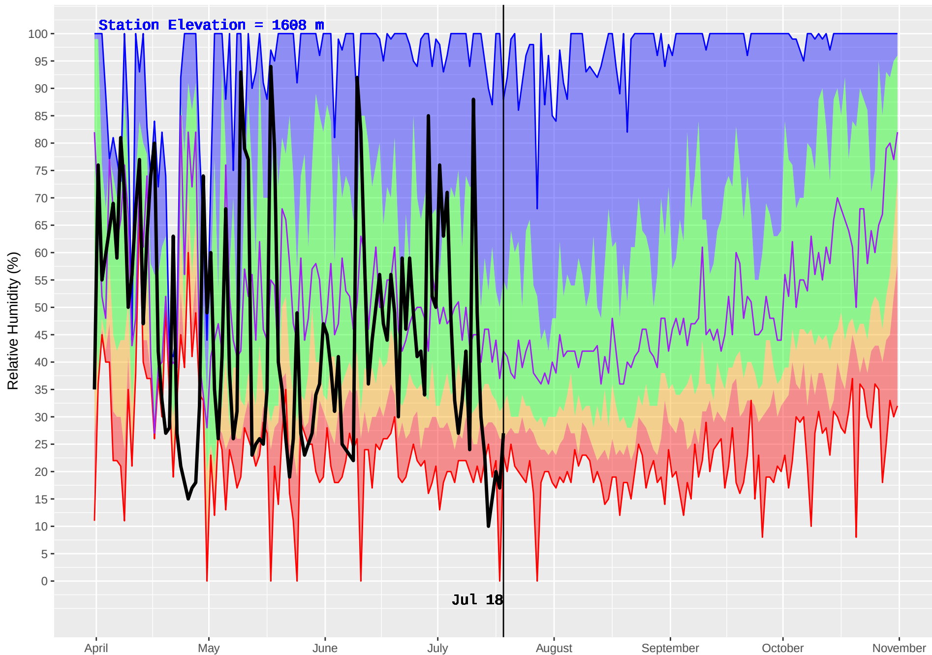
DEWAR CREEK (421) : Historical (1986–2016) and Current (2018) Daily Relative Humidity
